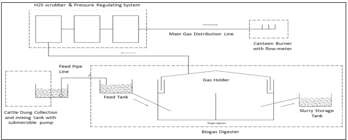
Biogas flow diagram
